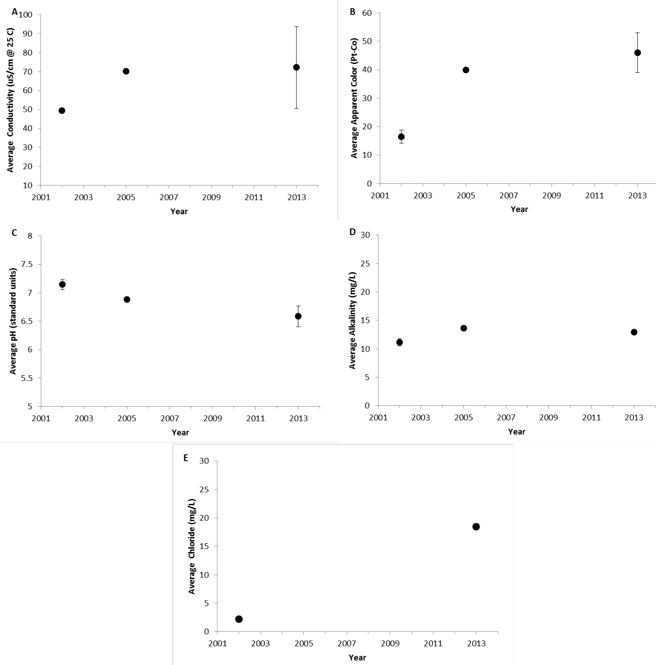
Figure 4. The annual average values of water quality indicators of Lake Clear, 2002-2013. (A) Specific lab conductivity @ 25°C, (B) apparent color, (C) pH, (D) total alkalinity, and (E) chloride concentration. Vertical bars represent one standard deviation of the mean.
