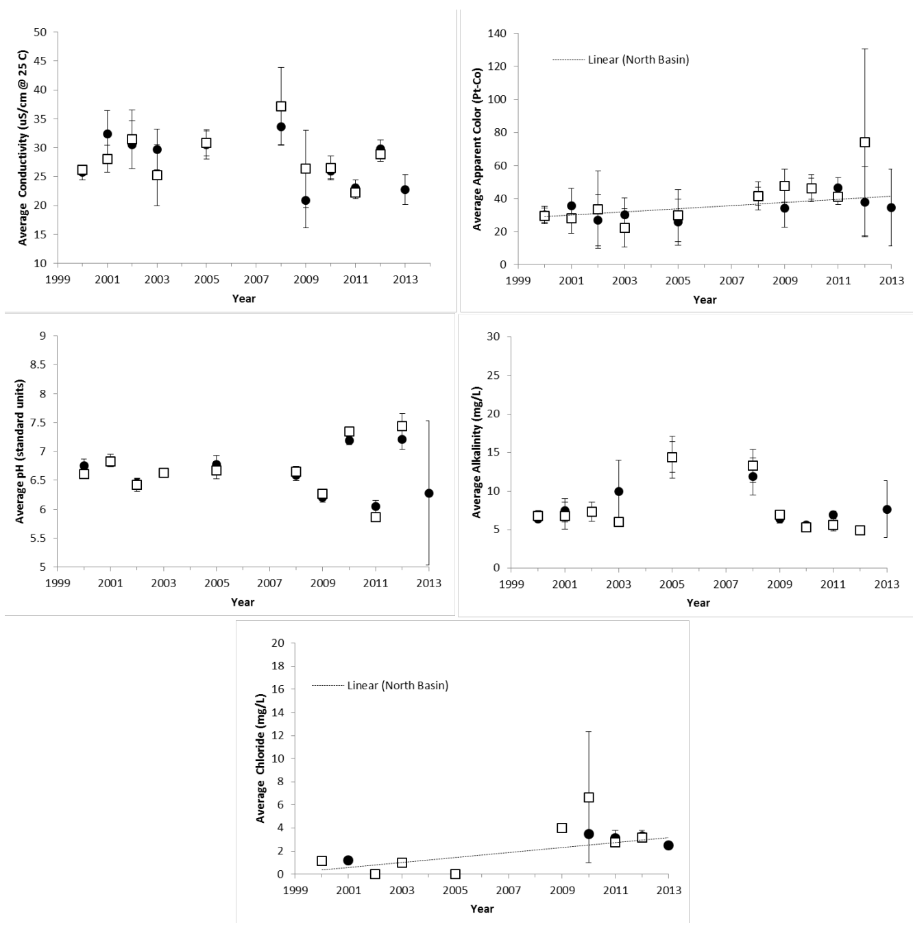
Figure 4. The annual average values of water quality indicators of Tupper Lake at the north and south basins, 2000-2013. (A) Specific lab conductivity @ 25°C, (B) apparent color, (C) pH, (D) total alkalinity, and (E) chloride concentration. Vertical bars represent one standard deviation of the mean. Significant trends ( P < 0.05 ) are noted with a trend line.
