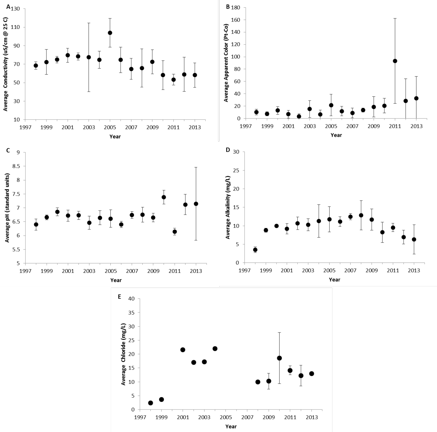
Figure 4. The annual average values of water quality indicators of Blue Mountain Lake, 1998-2013. (A) Specific lab conductivity @ 25°C, (B) apparent color, (C) pH, (D) total alkalinity, and (E) chloride concentration. Vertical bars represent one standard deviation of the lake wide mean. Significant trends ( P < 0.05 ) are noted with a trend line.
