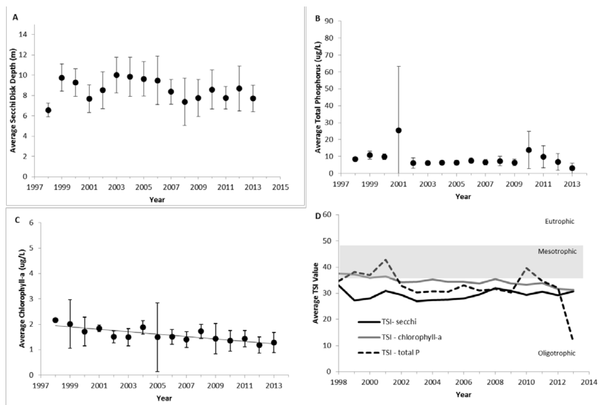
Figure 3. The annual average values of epilimnetic trophic indicators of Blue Mountain Lake, 1998-2013. (A) Secchi disk transparency, (B) total phosphorus concentration, (C) chlorophyll-a concentration, and (D) Carlson's Trophic State Index. Vertical bars represent one standard deviation of the lake wide mean. Significant trends ( P < 0.05 ) are noted with a trend line.
