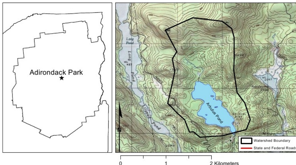
Figure 2. Location and watershed for Arbutus Lake.
