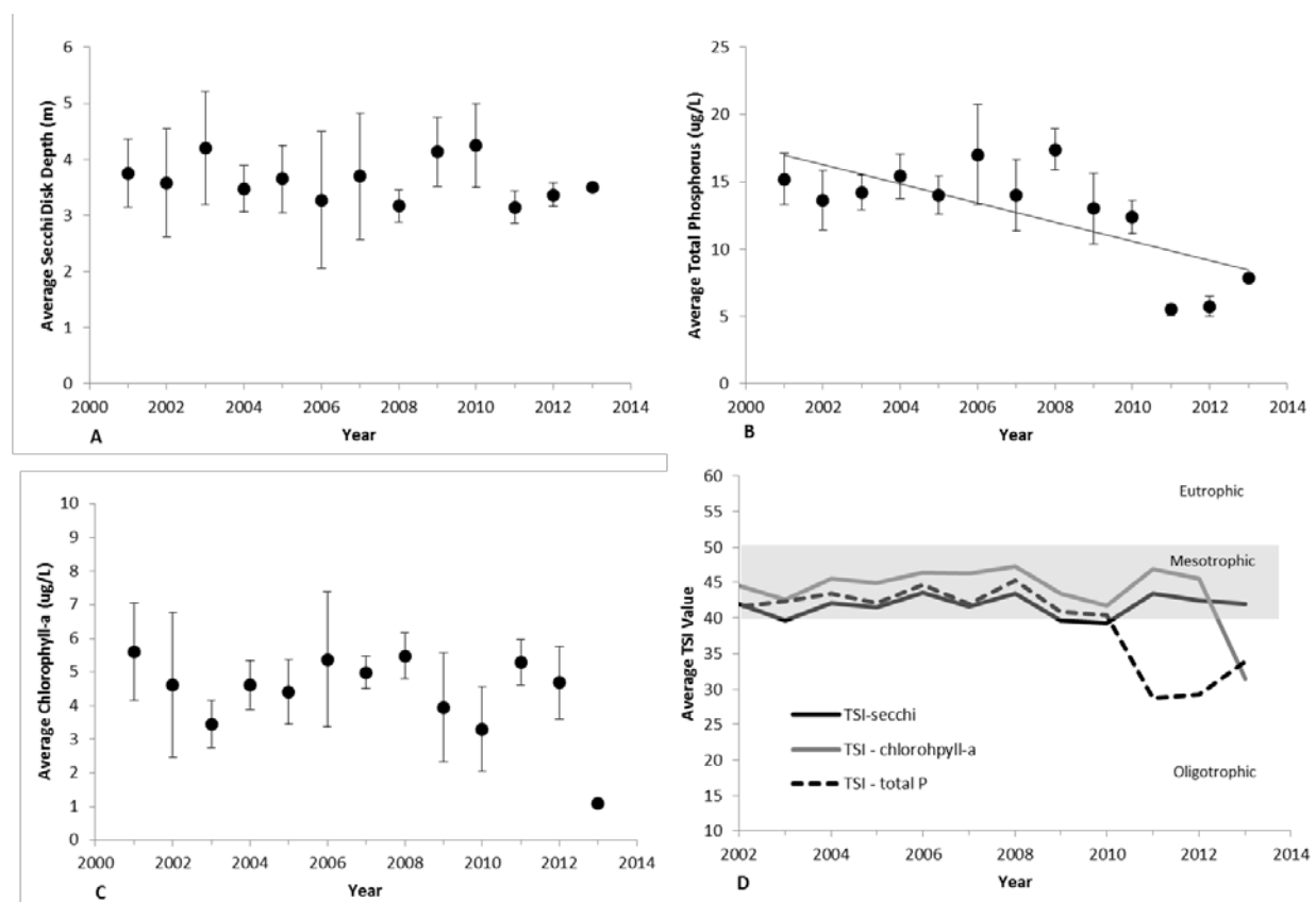
Figure 3. The annual average values of epilimnetic trophic indicators of Arbutus Lake, 2001-2013. (A) Secchi disk transparency, (B) total phosphorus concentration, (C) chlorophyll-a concentration, and (D) Carlson's Trophic State Index. Vertical bars represent one standard deviation of the mean. Significant trends ( P < 0.05 ) are noted with a trend line.
