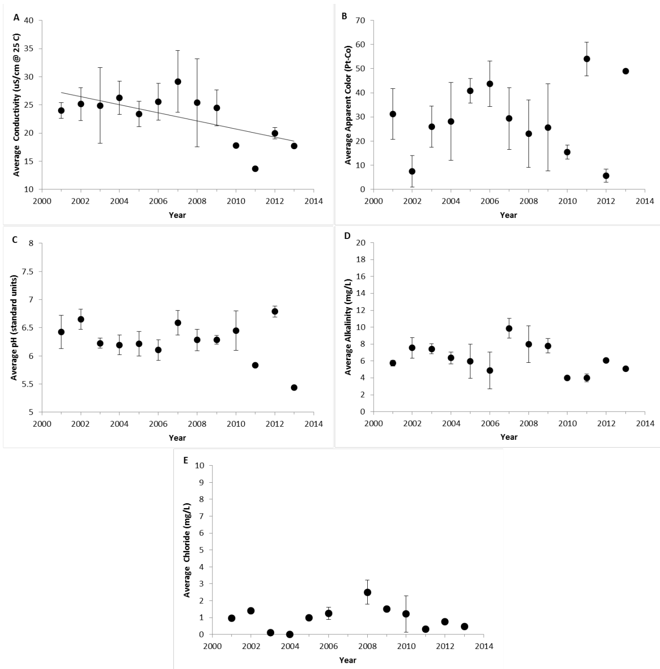
Figure 4. The annual average values of water quality indicators of Arbutus Lake, 2001-2013. (A) Specific lab conductivity @ 25°C, (B) apparent color, (C) pH, (D) total alkalinity, and (E) chloride concentration. Vertical bars represent one standard deviation of the mean. Significant trends ( P < 0.05 ) are noted with a trend line.
