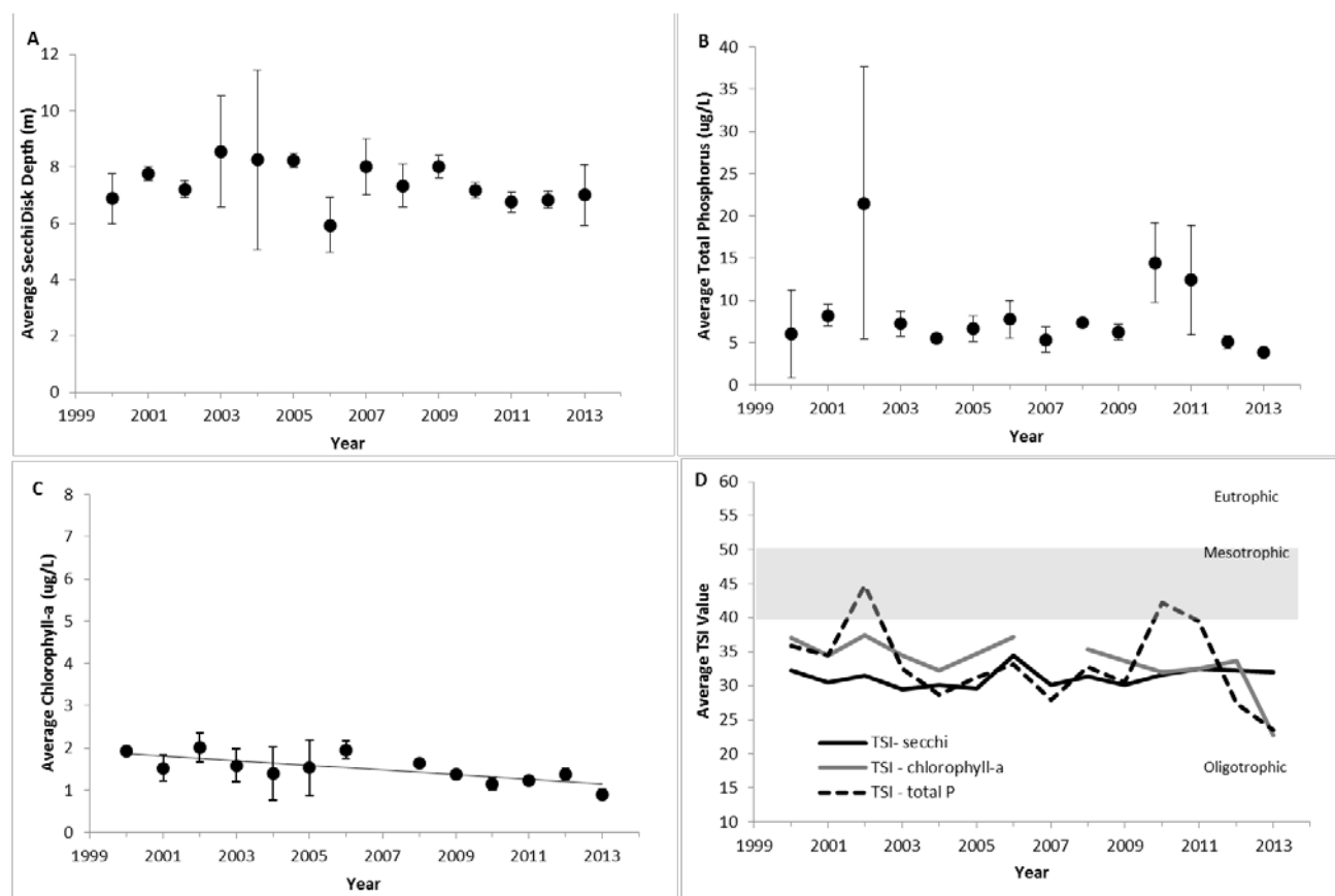
Figure 3. The annual average values of epilimnetic trophic indicators of White Lake, 2000-2013. (A) Secchi disk transparency, (B) total phosphorus concentration, (C) chlorophyll-a concentration, and (D) Carlson's Trophic State Index. Vertical bars represent one standard deviation of the mean. Significant trends ( P<0.05 ) are noted with a trend line.
