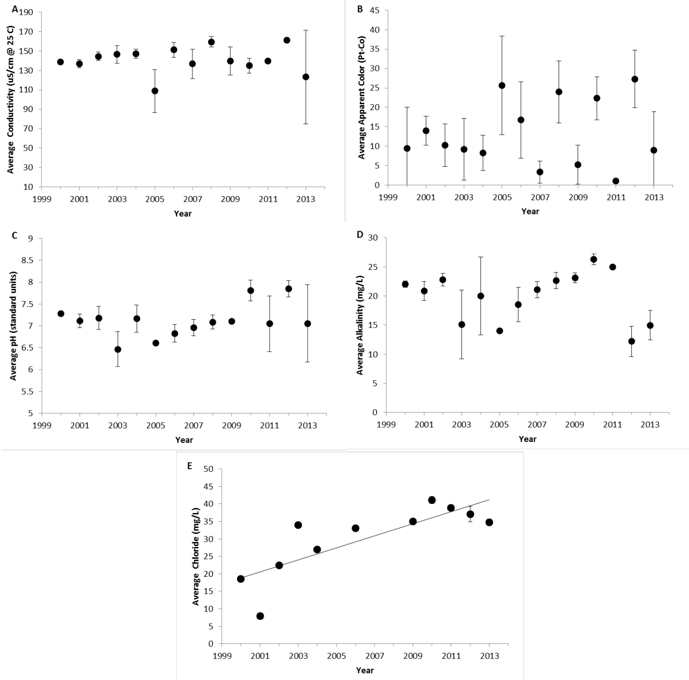
Figure 4. The annual average values of water quality indicators of White Lake, 2000-2013. (A) Specific lab conductivity @ 25°C, (B) apparent color, (C) pH, (D) total alkalinity, and (E) chloride concentration. Vertical bars represent one standard deviation of the mean. Significant trends ( P < 0.05 ) are noted with a trend line.
