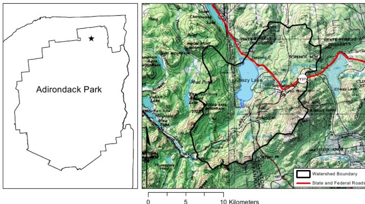
Figure 2. Location and watershed for Upper Chateaugay Lake.
