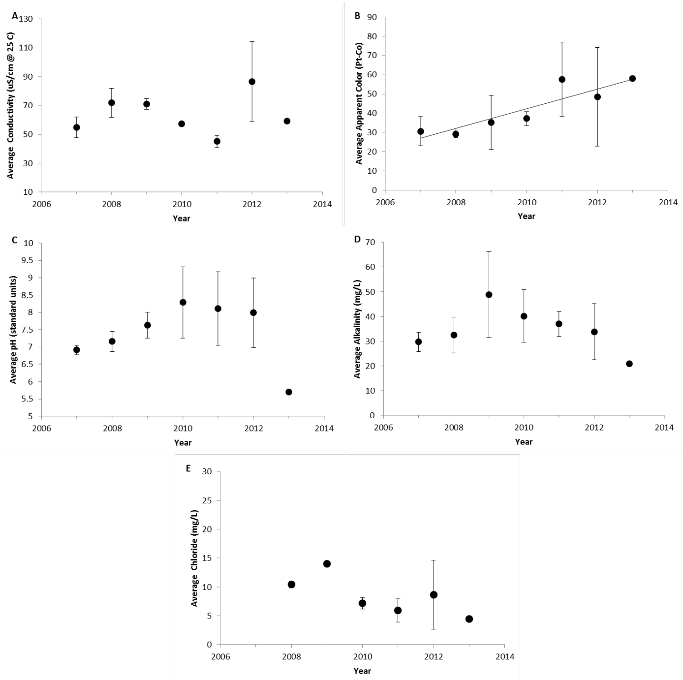
Figure 4. The annual average values of water quality indicators of Upper Chateaugay Lake, 2007-2013. (A) Specific lab conductivity @ 25°C, (B) apparent color, (C) pH, (D) total alkalinity, and (E) chloride concentration. Vertical bars represent one standard deviation of the mean. Significant trends ( P < 0.05 ) are noted with a trend line.
