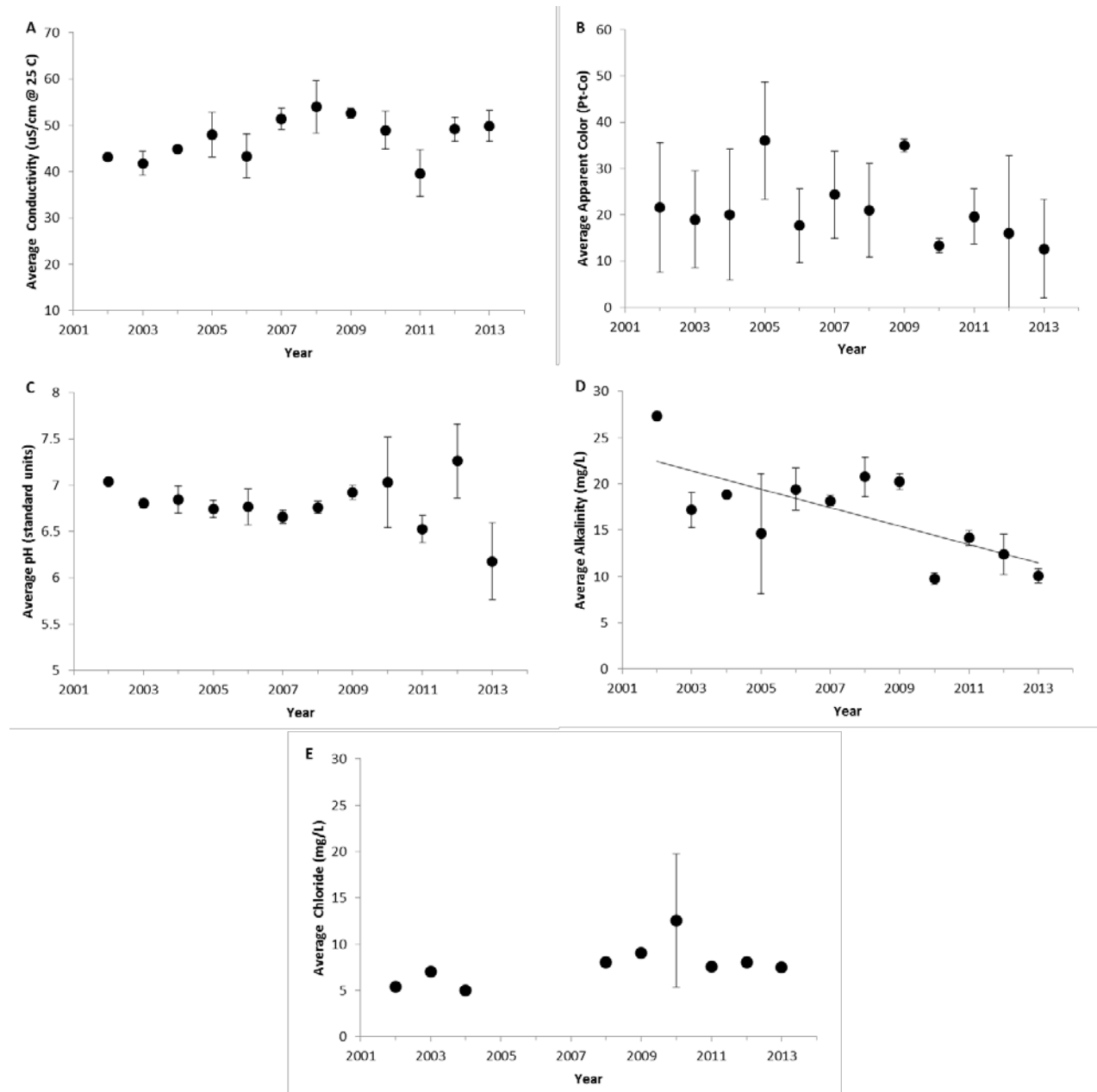
Figure 4. The annual average values of water quality indicators of Spitfire Lake, 2002-2013. (A) Specific lab conductivity @ 25°C, (B) apparent color, (C) pH, (D) total alkalinity, and (E) chloride concentration. Vertical bars represent one standard deviation of the mean. Significant trends ( P < 0.05 ) are noted with a trend line.
