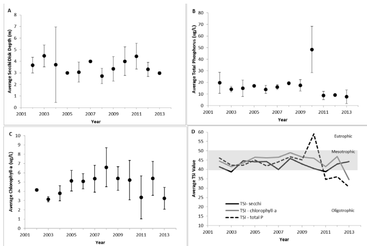
Figure 3. The annual average values of epilimnetic trophic indicators of Spitfire Lake, 2002-2013. (A) Secchi disk transparency, (B) total phosphorus concentration, (C) chlorophyll-a concentration, and (D) Carlson's Trophic State Index. Vertical bars represent one standard deviation of the mean. Significant trends ( P < 0.05 ) are noted with a trend line.
