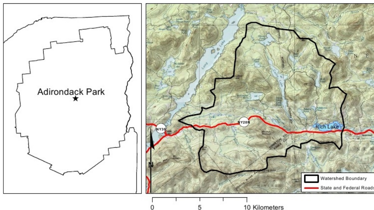
Figure 2. Location and watershed for Rich Lake.
