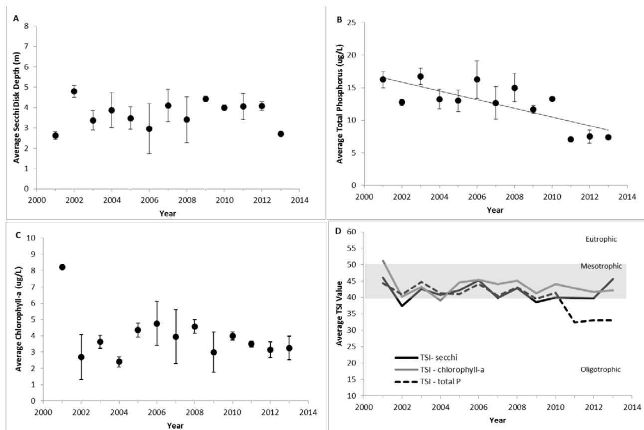
Figure 3. The annual average values of epilimnetic trophic indicators of Rich Lake, 2001-2013. (A) Secchi disk transparency, (B) total phosphorus concentration, (C) chlorophyll-a concentration, and (D) Carlson's Trophic State Index. Vertical bars represent one standard deviation of the mean. Significant trends ( P<0.05 ) are noted with a trend line.
