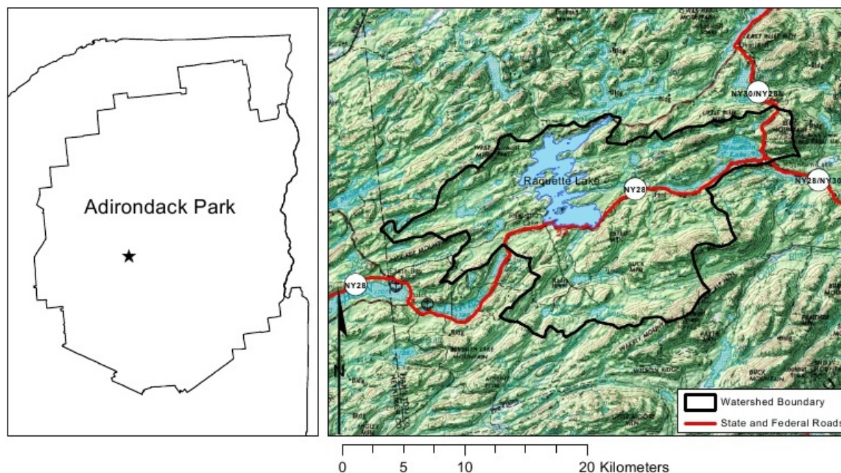
Figure 2. Location and watershed for Raquette Lake.
