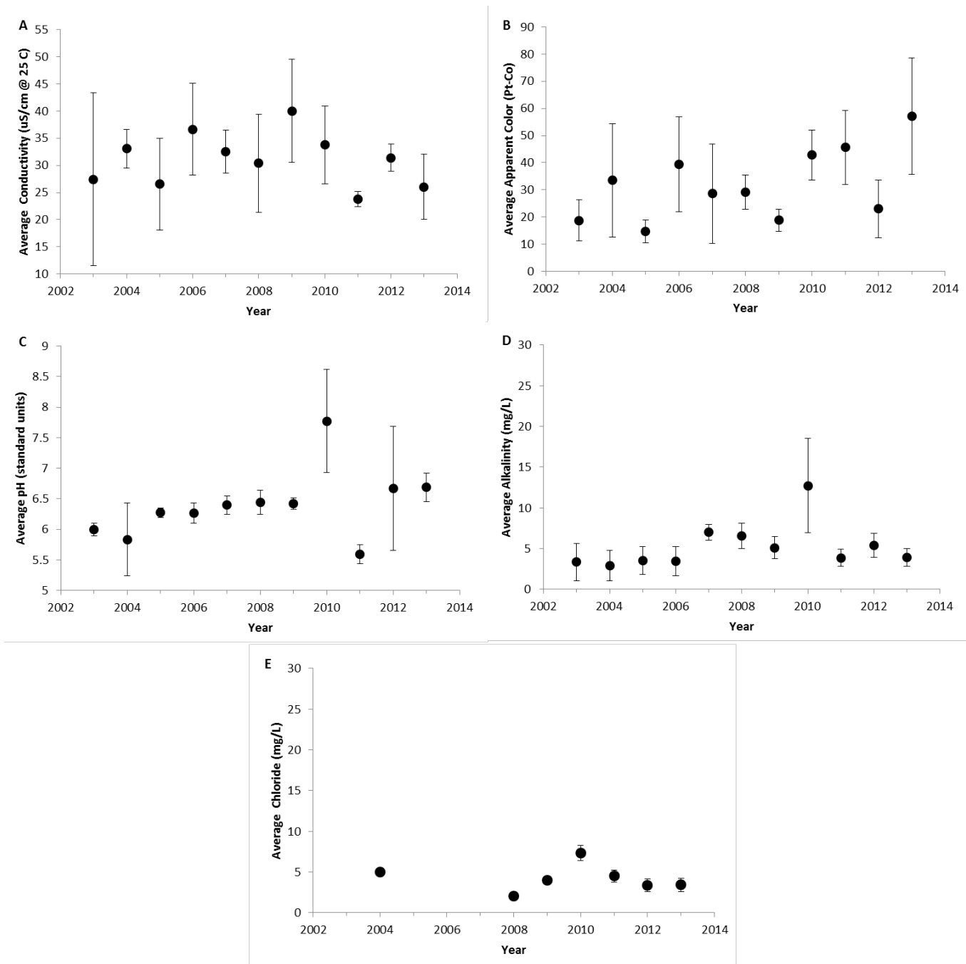
Figure 4. The annual average values of water quality indicators of Raquette Lake, 2003-2013. (A) Specific lab conductivity @ 25°C, (B) apparent color, (C) pH, (D) total alkalinity, and (E) chloride concentration. Vertical bars represent one standard deviation of the mean. Significant trends ( P < 0.05 ) are noted with a trend line.
