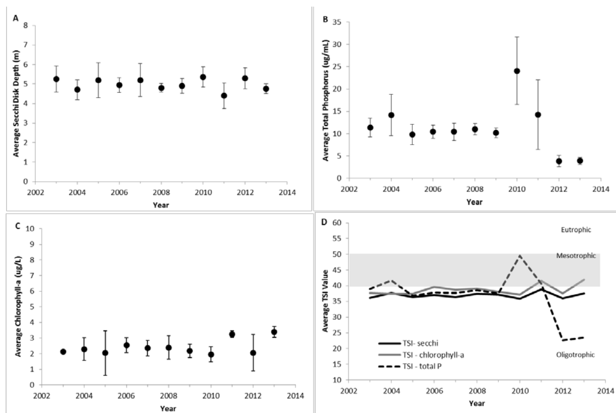
Figure 3. The annual average values of epilimnetic trophic indicators of Raquette Lake, 2003-2013. (A) Secchi disk transparency, (B) total phosphorus concentration, (C) chlorophyll-a concentration, and (D) Carlson's Trophic State Index. Vertical bars represent one standard deviation of the mean. Significant trends ( P < 0.05 ) are noted with a trend line.
