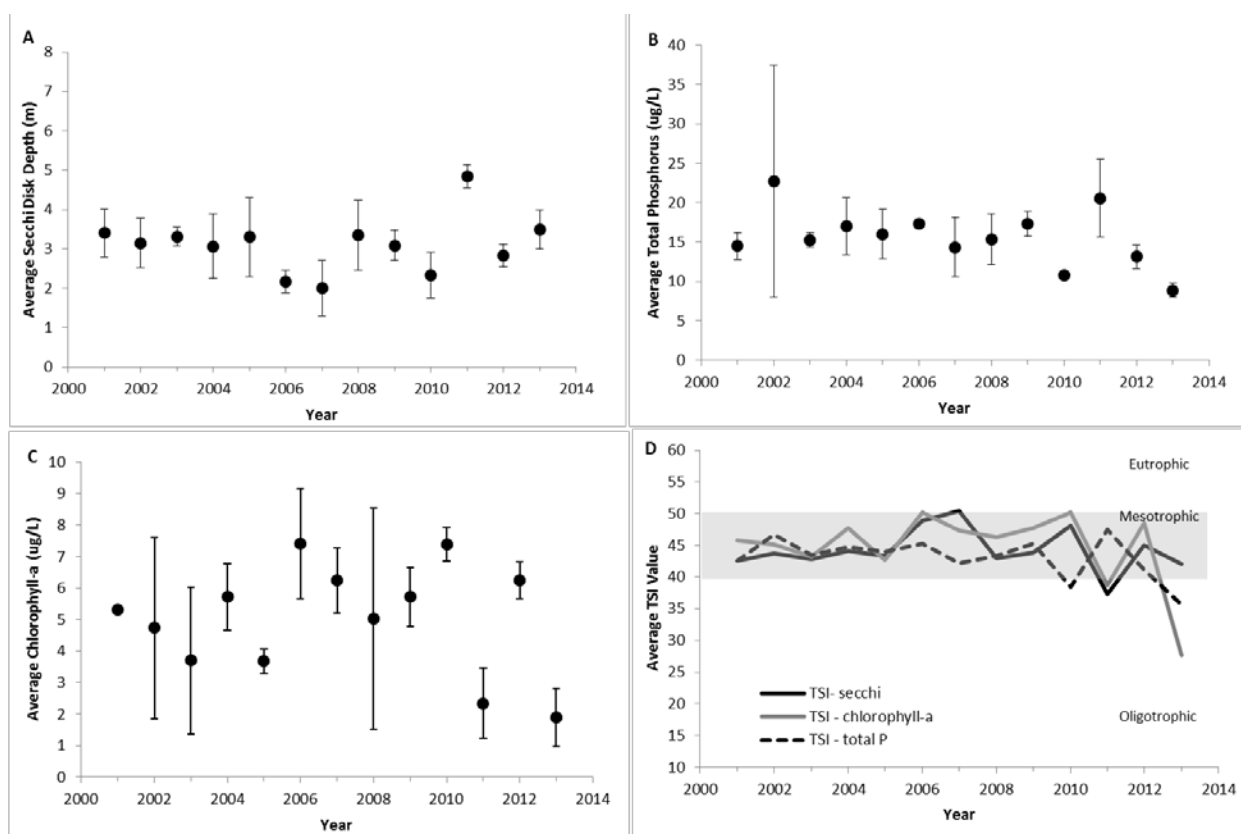
Figure 3. The annual average values of epilimnetic trophic indicators of Long Pond, 2001-2013. (A) Secchi disk transparency, (B) total phosphorus concentration, (C) chlorophyll-a concentration, and (D) Carlson's Trophic State Index. Vertical bars represent one standard deviation of the mean. Significant trends ( P < 0.05 ) are noted with a trend line.
