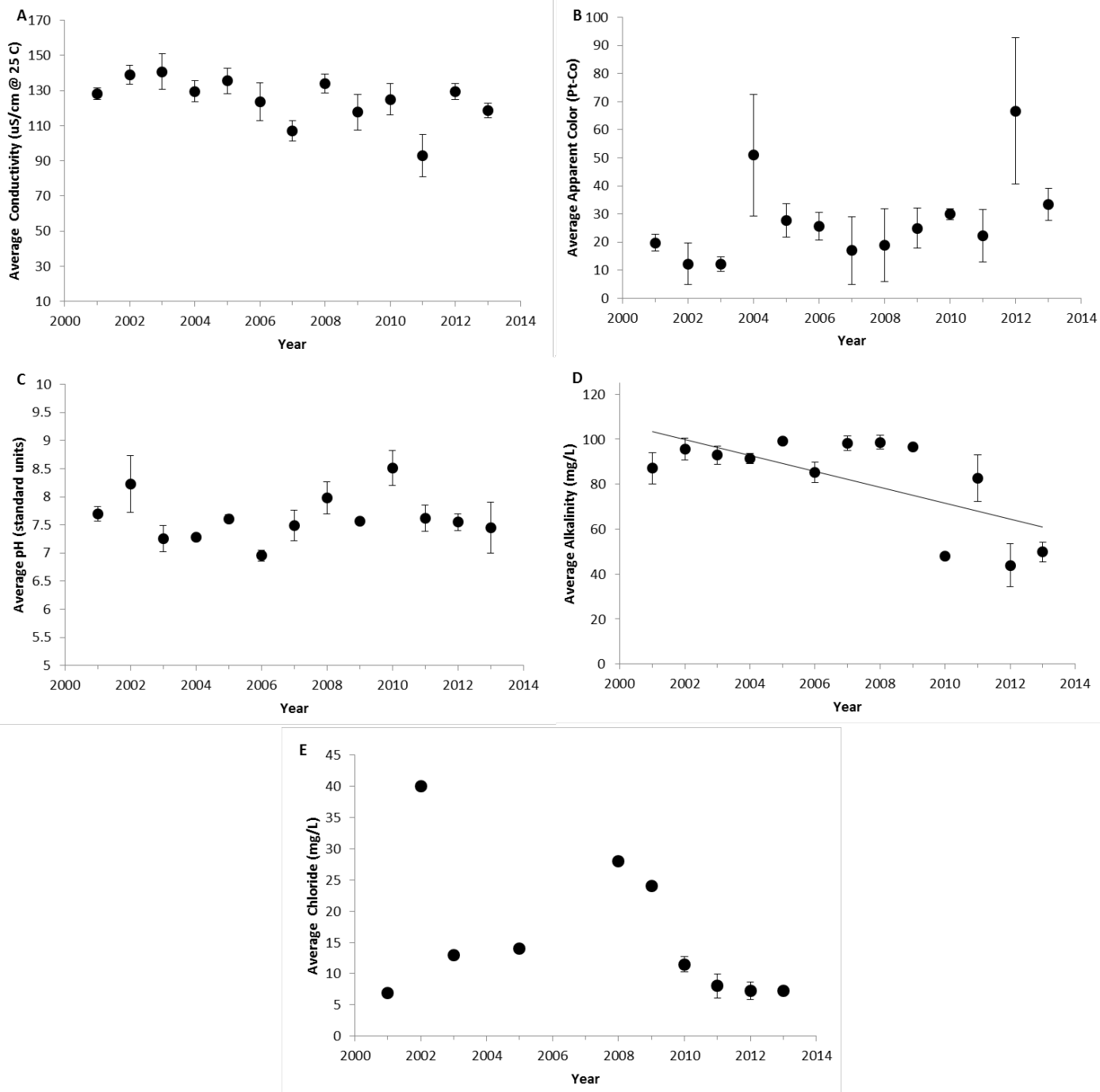
Figure 4. The annual average values of water quality indicators of Long Pond, 2001-2013. (A) Specific lab conductivity @ 25°C, (B) apparent color, (C) pH, (D) total alkalinity, and (E) chloride concentration. Vertical bars represent one standard deviation of the mean. Significant trends ( P < 0.05 ) are noted with a trend line.
