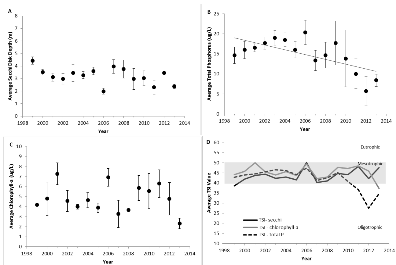
Figure 3. The annual average values of epilimnetic trophic indicators of Little Long Lake, 1999-2013. (A) Secchi disk transparency, (B) total phosphorus concentration, (C) chlorophyll-a concentration, and (D) Carlson's Trophic State Index. Vertical bars represent one standard deviation of the mean. Significant trends ( P < 0.05 ) are noted with a trend line.
