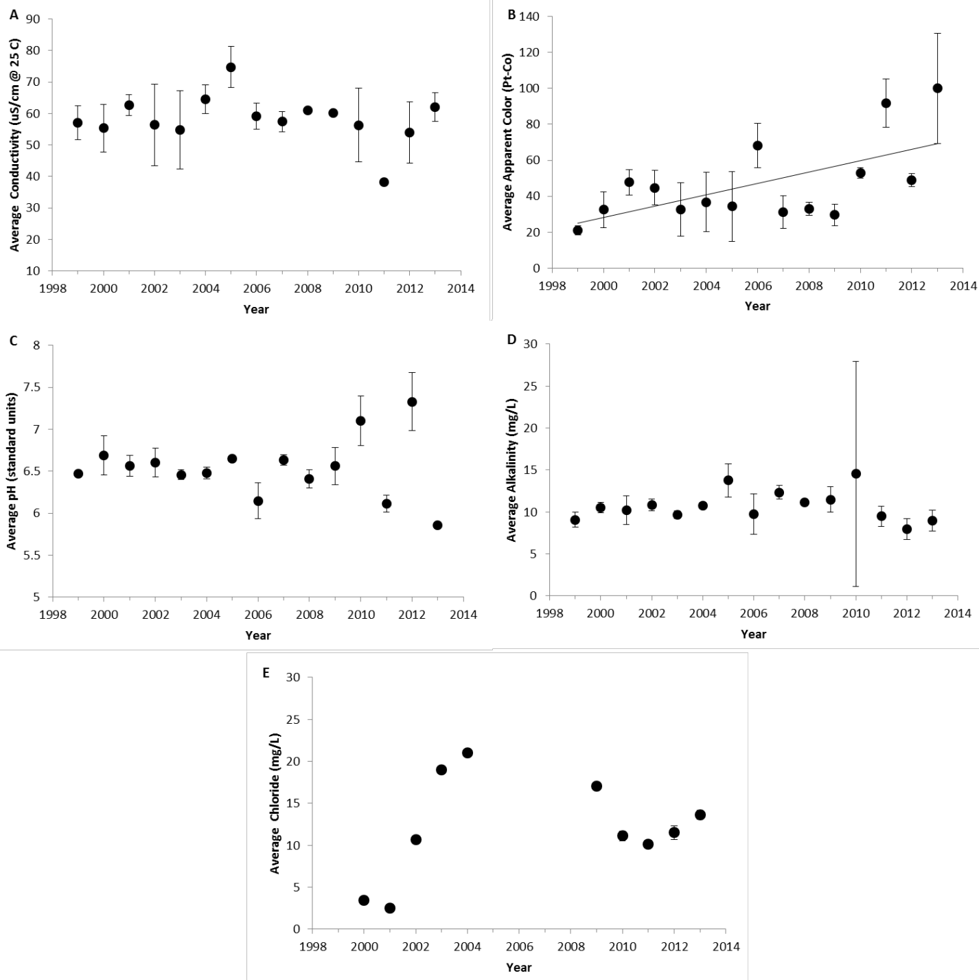
Figure 4. The annual average values of water quality indicators of Little Long Lake, 1999-2013. (A) Specific lab conductivity @ 25°C, (B) apparent color, (C) pH, (D) total alkalinity, and (E) chloride concentration. Vertical bars represent one standard deviation of the mean. Significant trends ( P < 0.05 ) are noted with a trend line.
