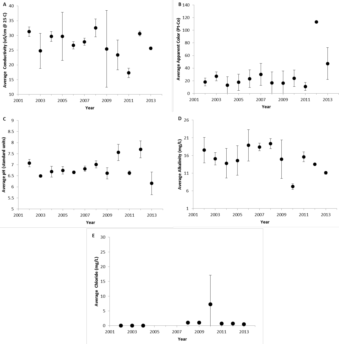
Figure 4. The annual average values of water quality indicators of Garnet Lake, 2002-2013. (A) Specific lab conductivity @ 25°C, (B) apparent color, (C) pH, (D) total alkalinity, and (E) chloride concentration. Vertical bars represent one standard deviation of the mean. Significant trends ( P < 0.05 ) are noted with a trend line.
