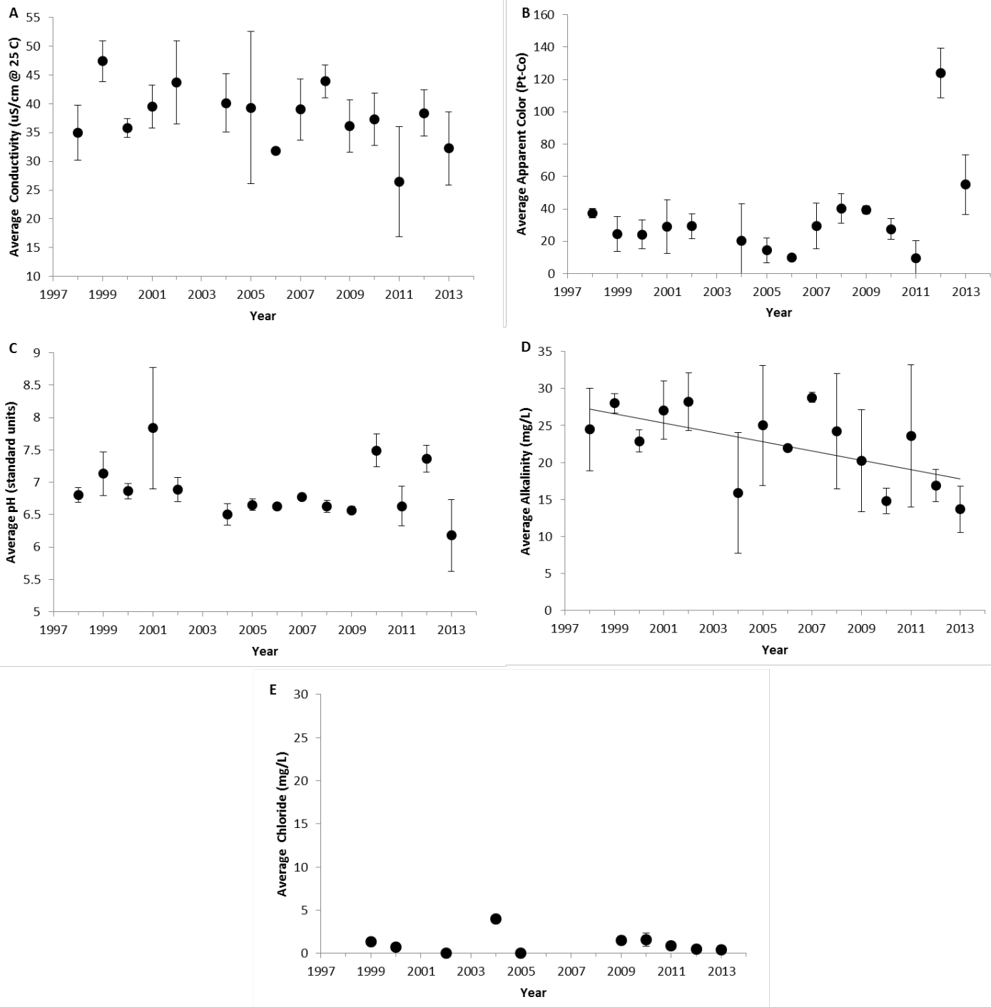
Figure 4. The annual average values of water quality indicators of Eli Pond, 1998-2013. (A) Specific lab conductivity @ 25°C, (B) apparent color, (C) pH, (D) total alkalinity, and (E) chloride concentration. Vertical bars represent one standard deviation of the mean. Significant trends ( P < 0.05 ) are noted with a trend line.
