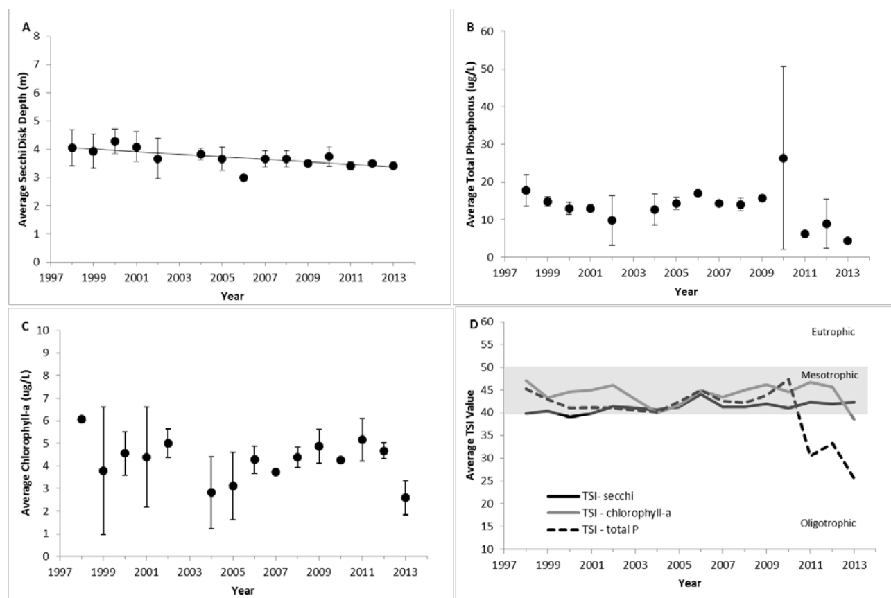
Figure 3. The annual average values of epilimnetic trophic indicators of Eli Pond, 1998-2013. (A) Secchi disk transparency, (B) total phosphorus concentration, (C) chlorophyll-a concentration, and (D) Carlson's Trophic State Index. Vertical bars represent one standard deviation of the mean. Significant trends ( P < 0.05 ) are noted with a trend line.
