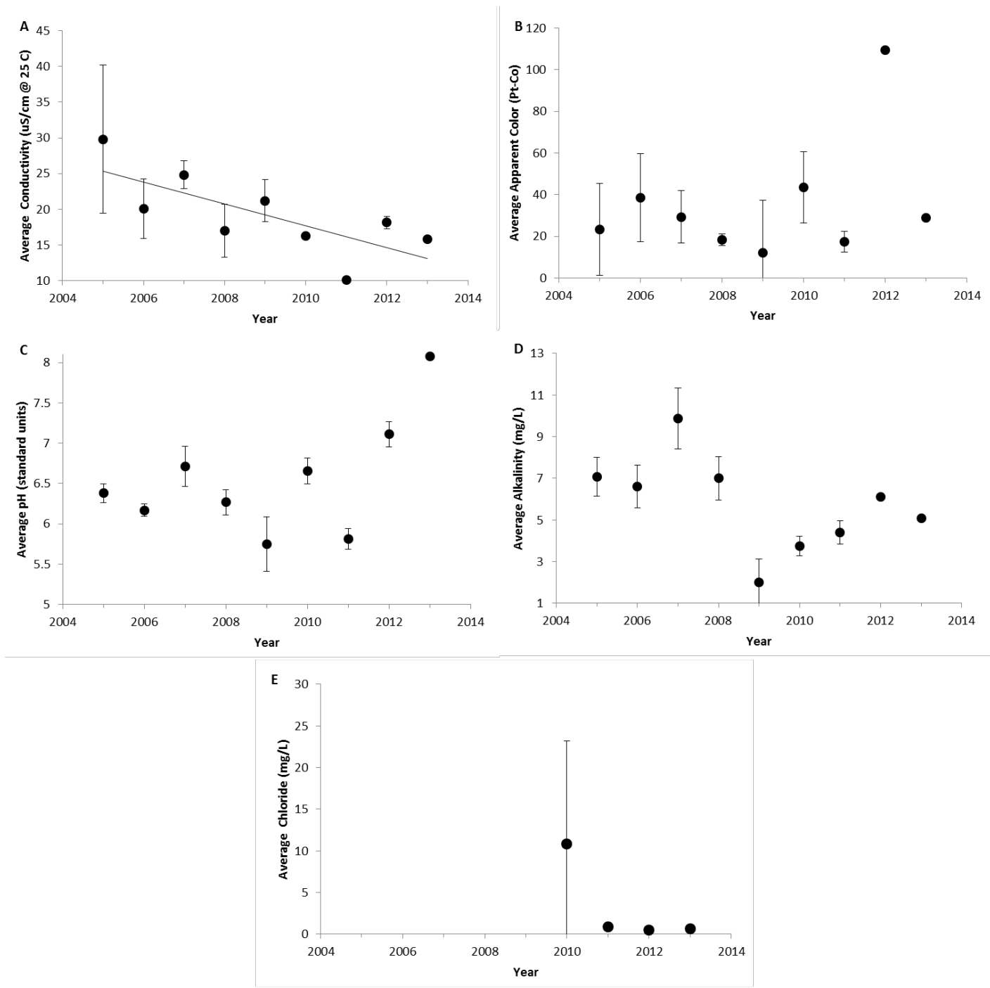
Figure 4. The annual average values of water quality indicators of Dug Mountain Pond, 2005-2013. (A) Specific lab conductivity @ 25°C, (B) apparent color, (C) pH, (D) total alkalinity, and (E) chloride concentration. Vertical bars represent one standard deviation of the mean. Significant trends ( P < 0.05 ) are noted with a trend line.
