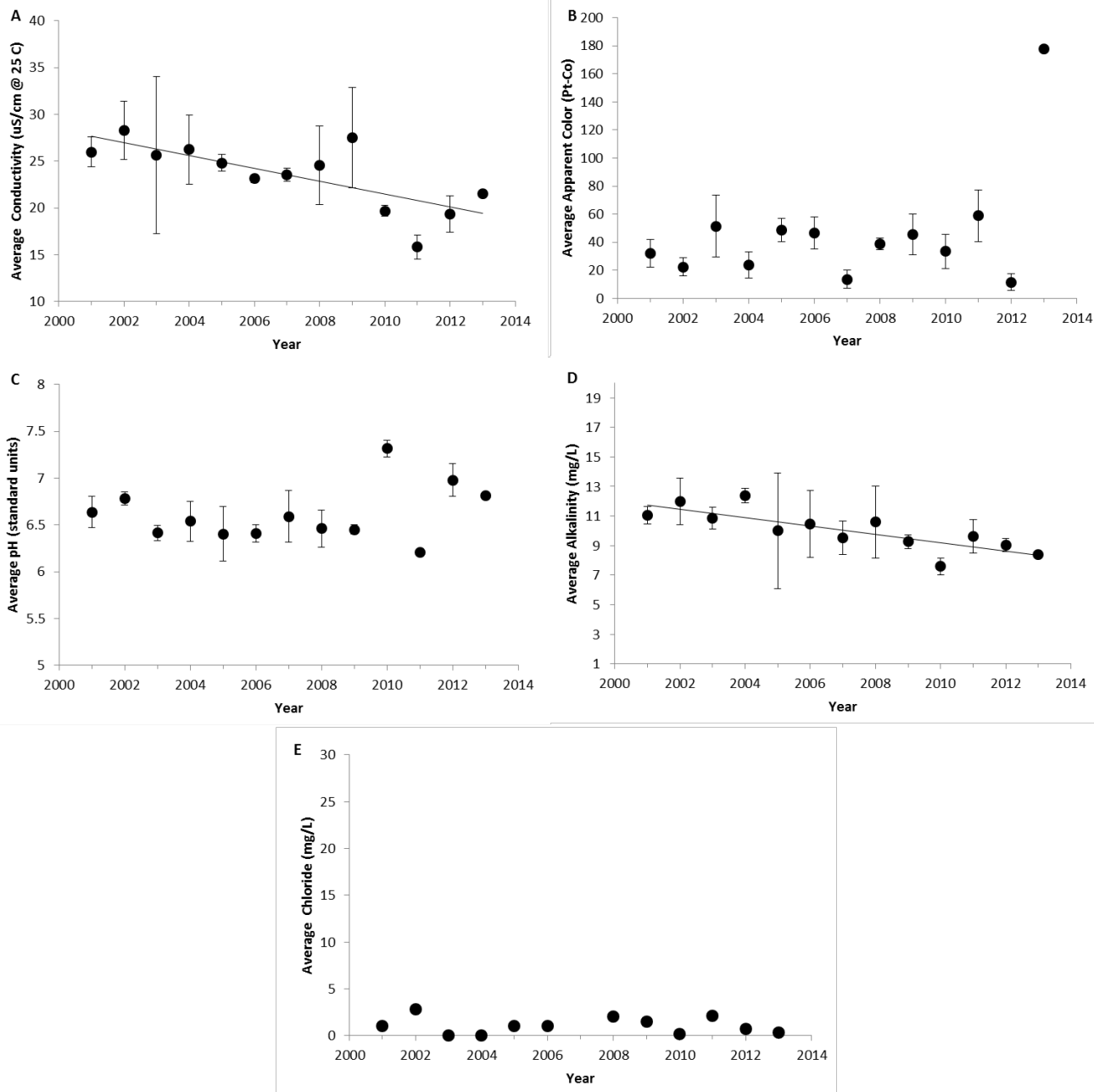
Figure 4. The annual average values of water quality indicators of Deer Lake, 2001-2013. (A) Specific lab conductivity @ 25°C, (B) apparent color, (C) pH, (D) total alkalinity, and (E) chloride concentration. Vertical bars represent one standard deviation of the mean. Significant trends ( P<0.05 ) are noted with a trend line.
