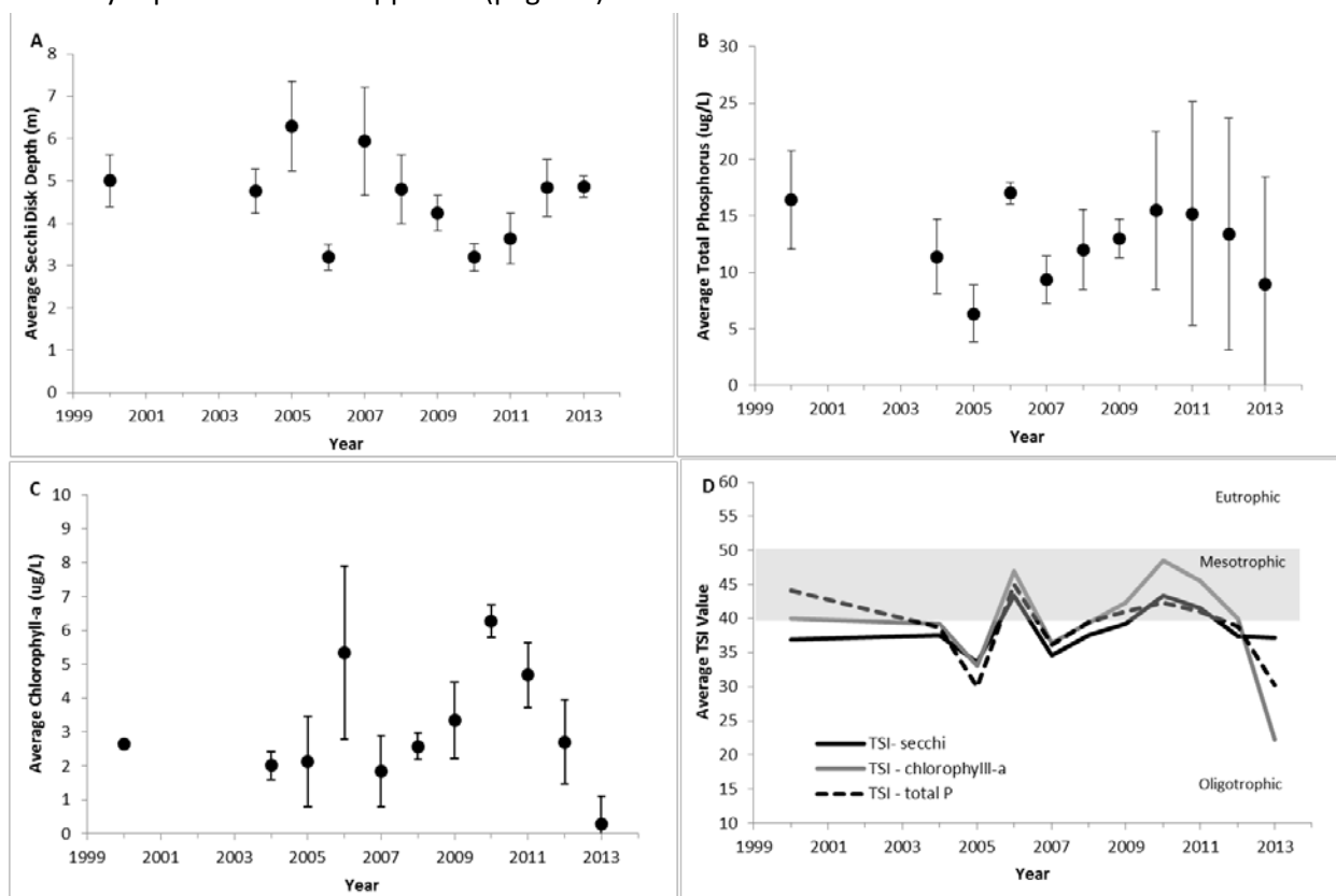
Figure 3. The annual average values of epilimnetic trophic indicators of Canada Lake, 2000-2013. (A) Secchi disk transparency, (B) total phosphorus concentration, (C) chlorophyll-a concentration, and (D) Carlson's Trophic State Index. Vertical bars represent one standard deviation of the mean. Significant trends ( P < 0.05 ) are noted with a trend line.
