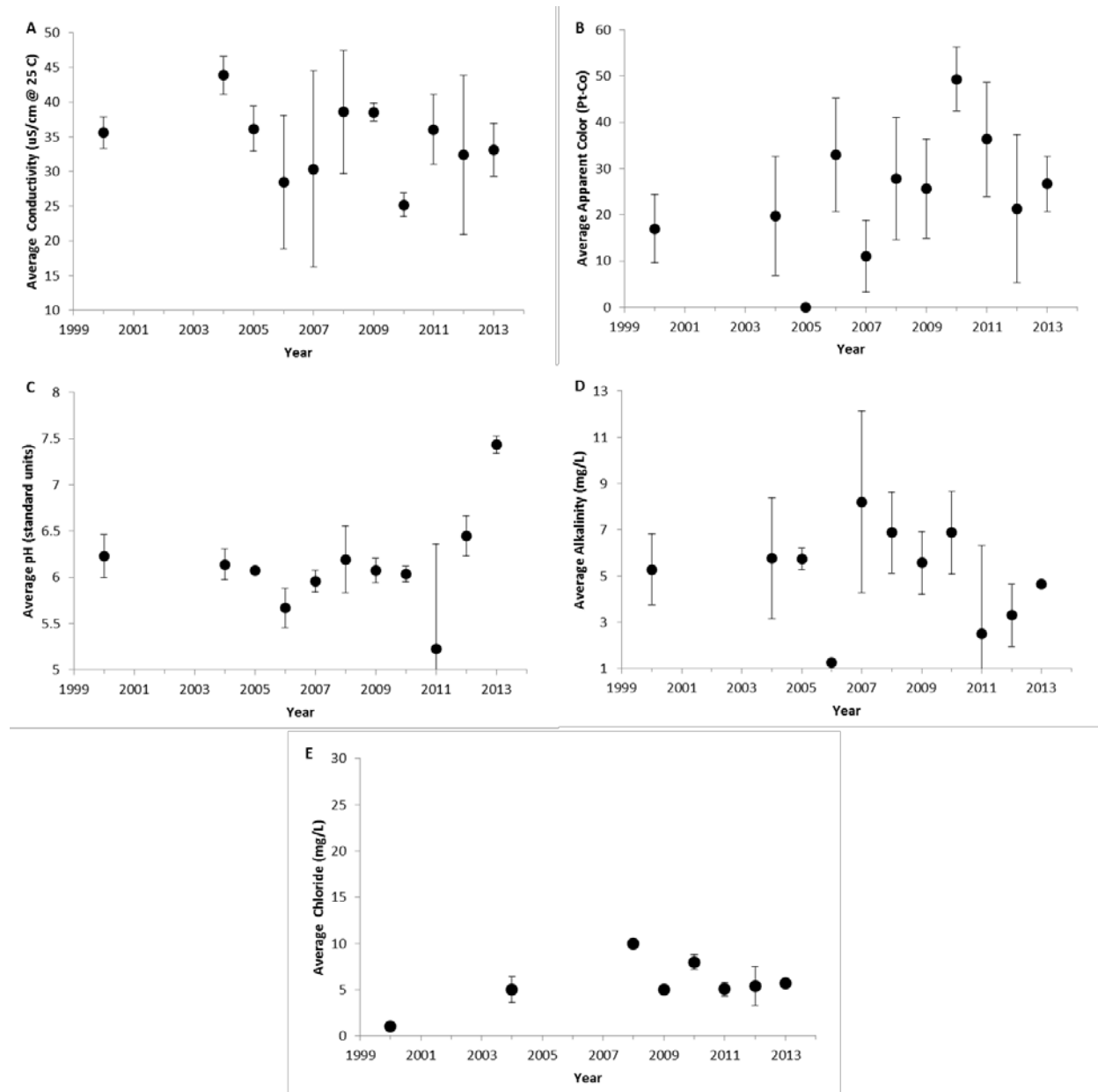
Figure 4. The annual average values of water quality indicators of Canada Lake, 2000-2013. (A) Specific lab conductivity @ 25°C, (B) apparent color, (C) pH, (D) total alkalinity, and (E) chloride concentration. Vertical bars represent one standard deviation of the mean. Significant trends ( P < 0.05 ) are noted with a trend line.
